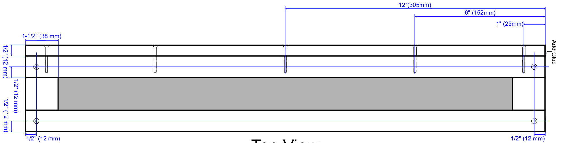
Top View
