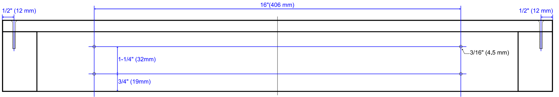
Front View
