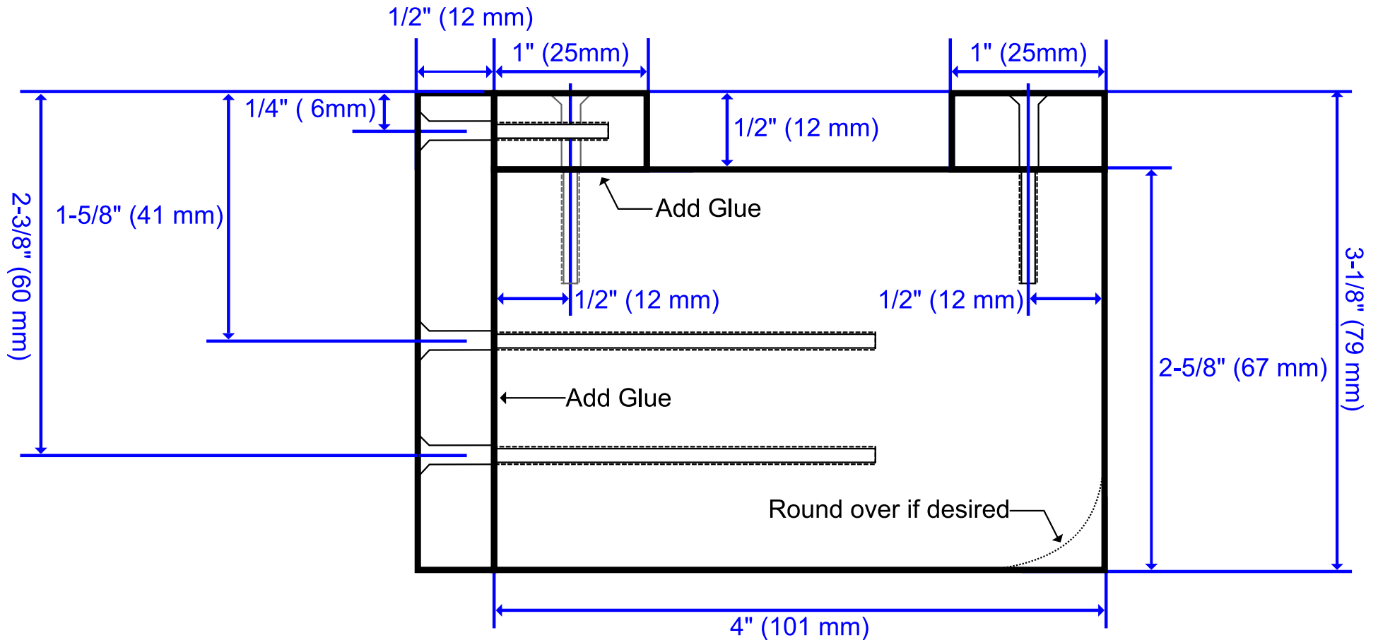
Side View
